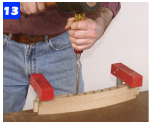
13 Securely clamp a rail to the worktable, square the mortise walls and remove the remaining waste.
